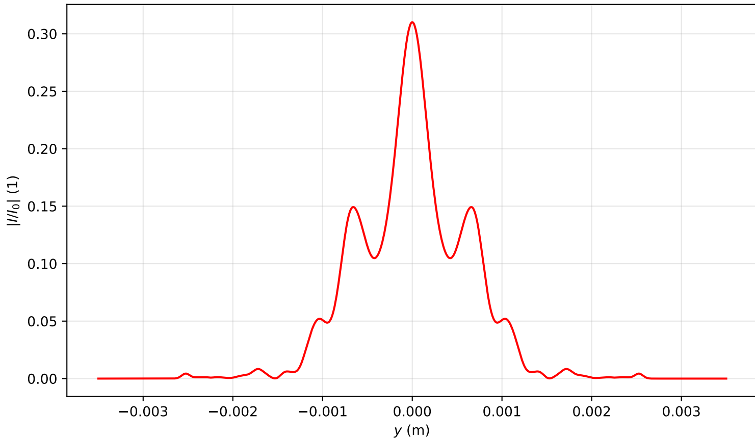
Intensity profile I(x=0, y, z=1.911)/I_0 , P_{in}=6.5P_{cr} , artificial time
